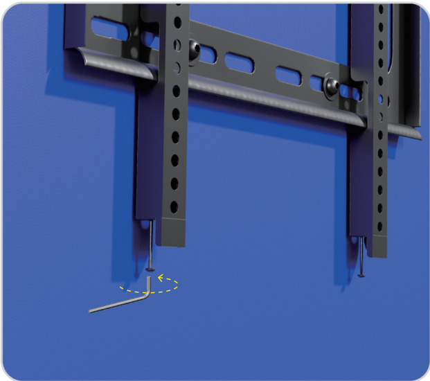
Use a wrench to tighten the fixing screws of the brackets. The TV rack installation is now complete.
