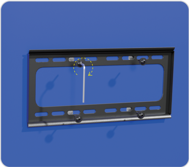
Secure the wall plate to the shelf with screws. Pre-drilled holes are provided at the corresponding positions on the graphic.
