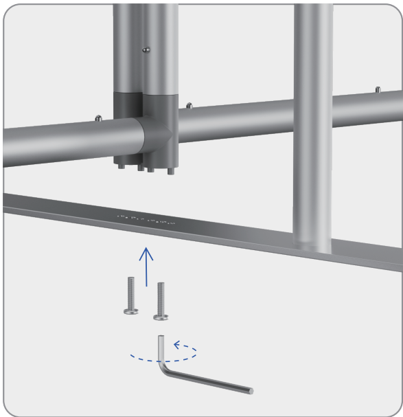
Align the stands side by side. Secure them to the modular table kit's base using screws.
