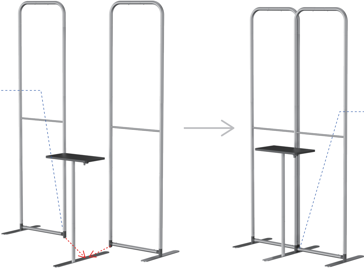
Remove the original base from both display stands.
